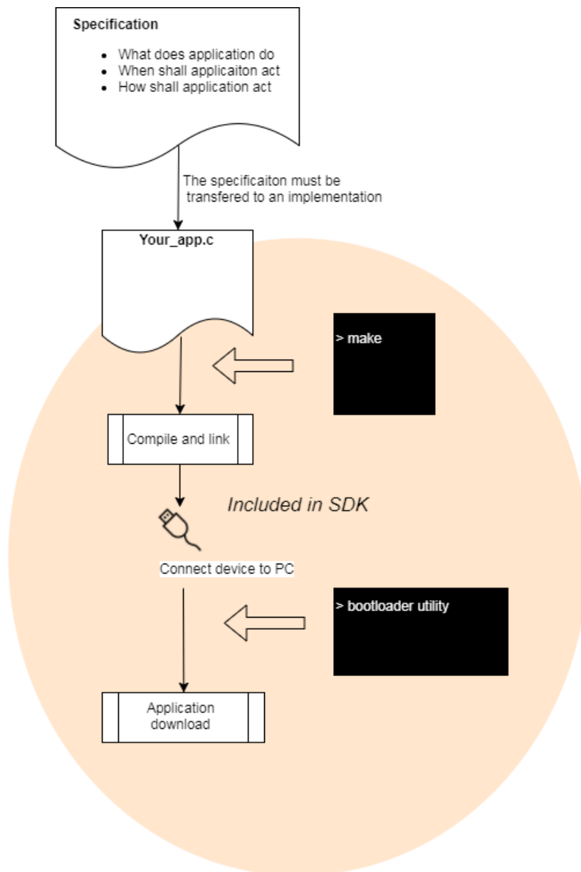
Figure 3. Workflow using RIIM SDK
