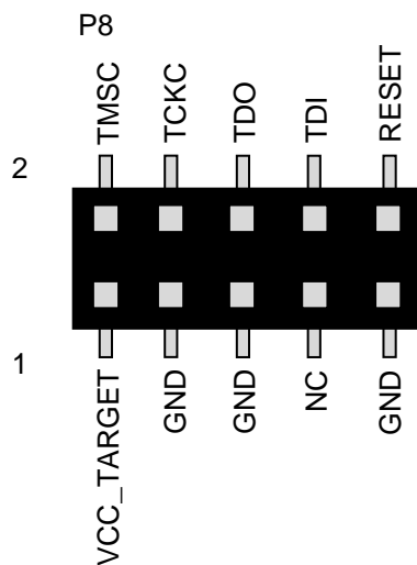
Figure 5. Programming connector P8
